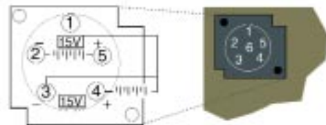
Connector Pin Schematic
